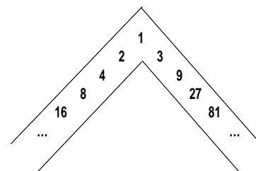
Figure 9. Pythagorean Lambda
